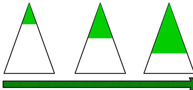
Top-Down-Strategie
